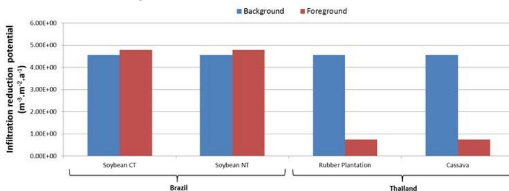
Figure 2. Characterization factor values for infiltration reduction potential occupation impact.
