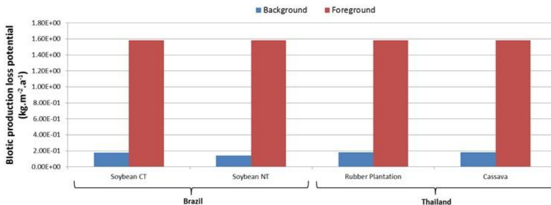
Figure 5. Characterization factor values for biotic production loss potential occupation impact
