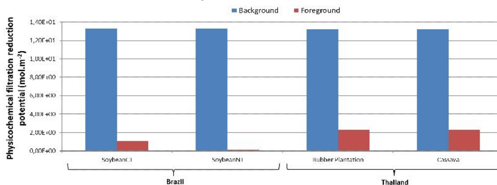
Figure 1. Characterization factor values for erosion potential occupation impact.
