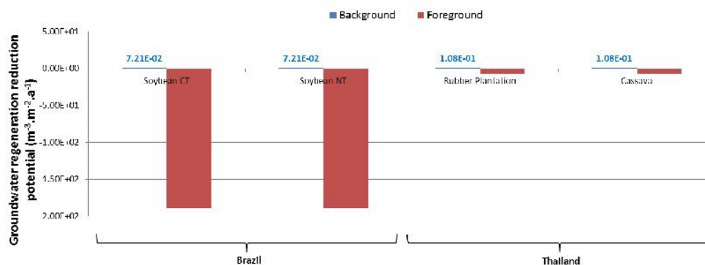
Figure 4. Characterization factor values for groundwater regeneration reduction occupation impact
