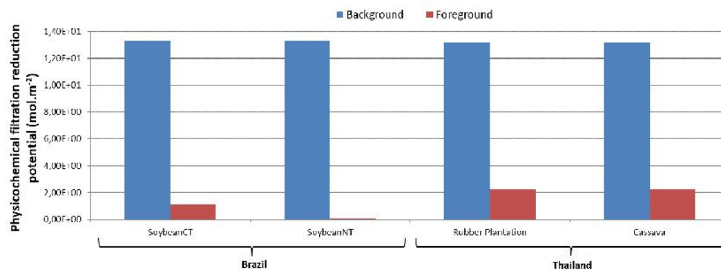
Figure 3. Characterization factor values for physicochemical filtration reduction potential occupation impact.
