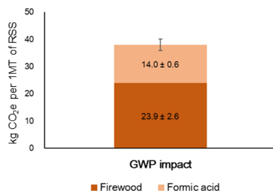
Fig. 4. Global warming potential (GWP) of ribbed smoked sheet manufacture (RSS) per 1 MT of RSS. All values are denoted as mean \pm standard error in kg CO 2 e per 1 MT of RSS.
